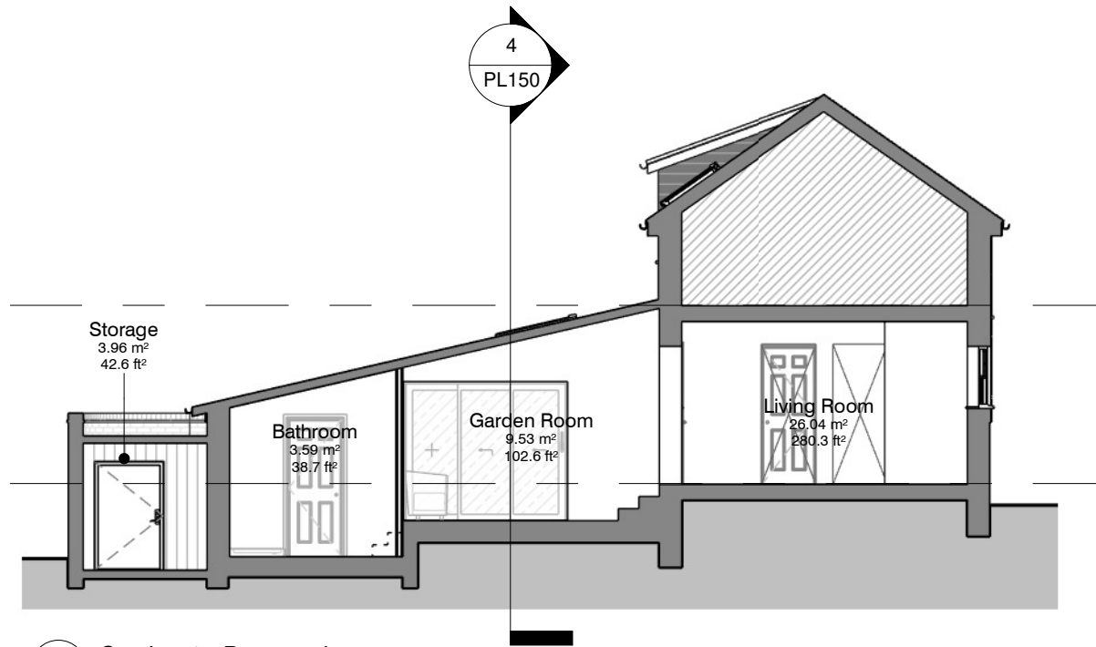
2 Section 1 - Proposed 1 : 100 @A3
