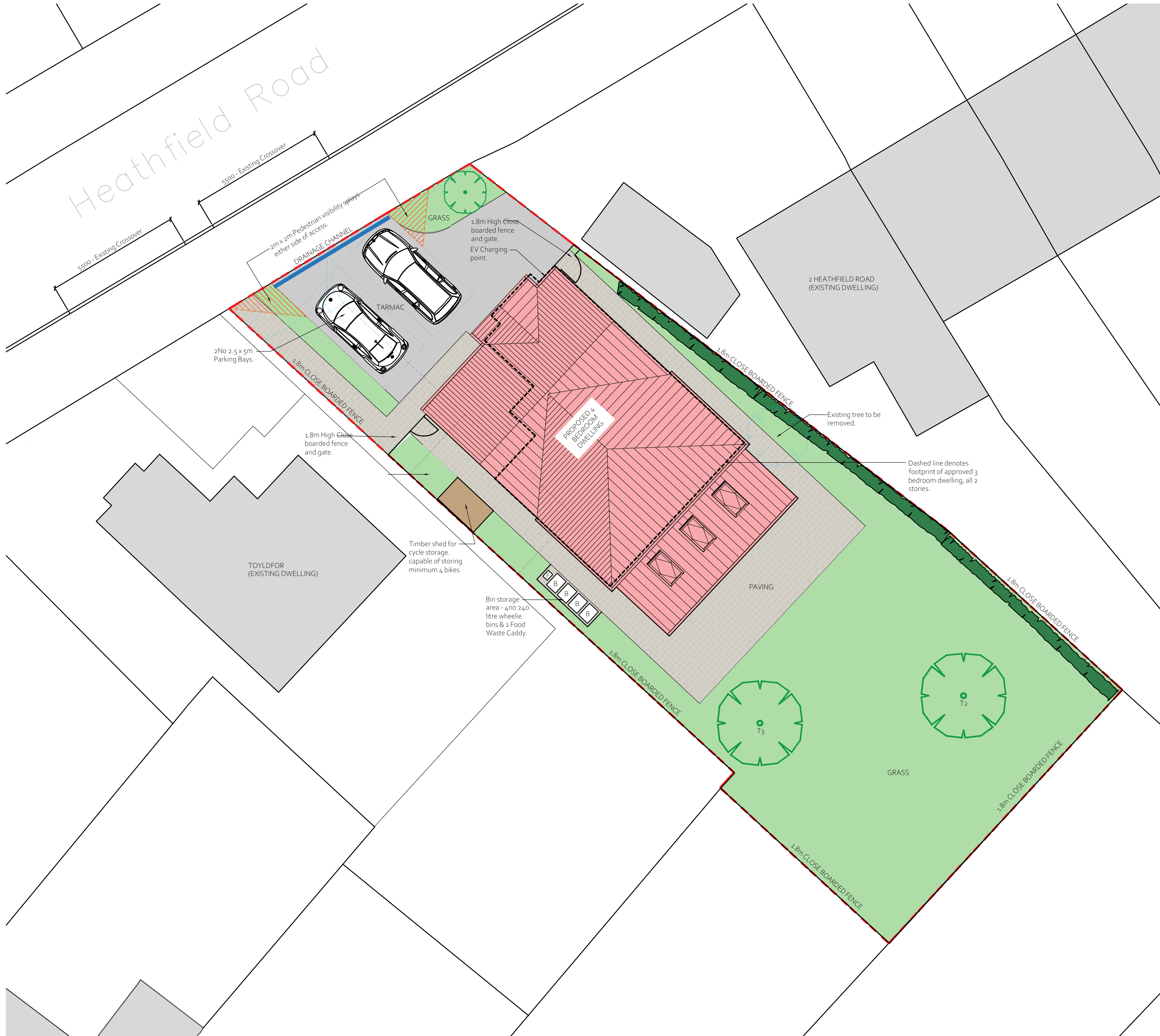
PROPOSED BLOCK PLAN @ 1 TO 100
