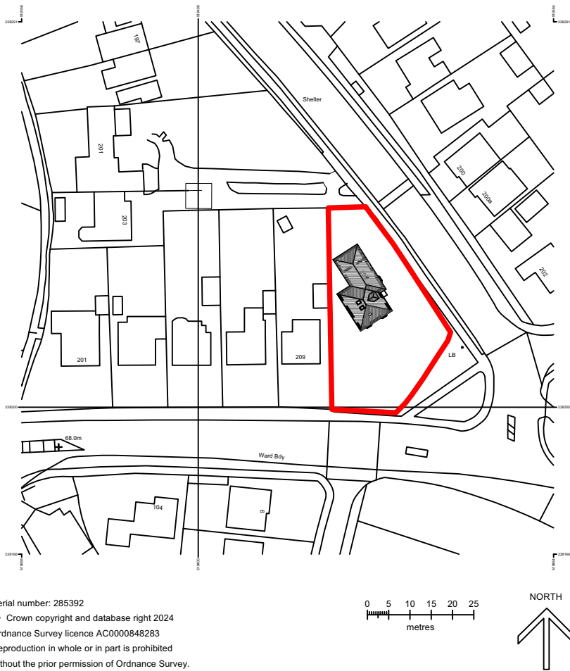
EXISTING SITE LOCATION 1:500
