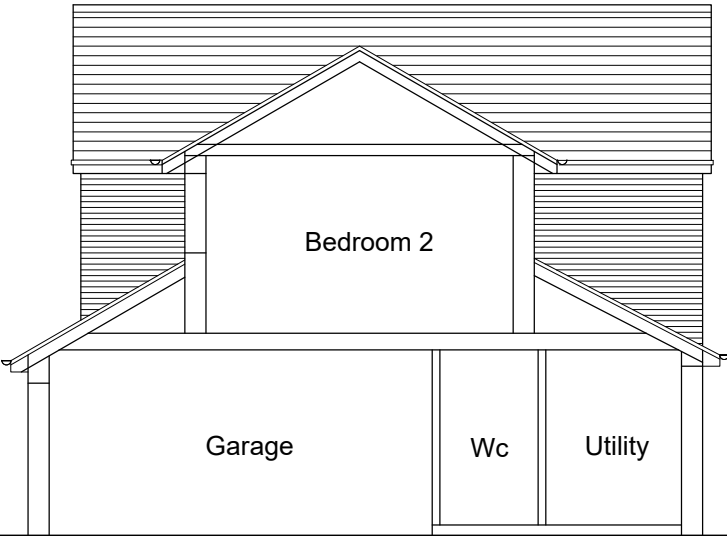
Existing Section A-A
