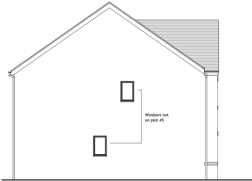
Left Elevation
