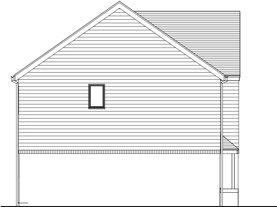
Left Elevation
