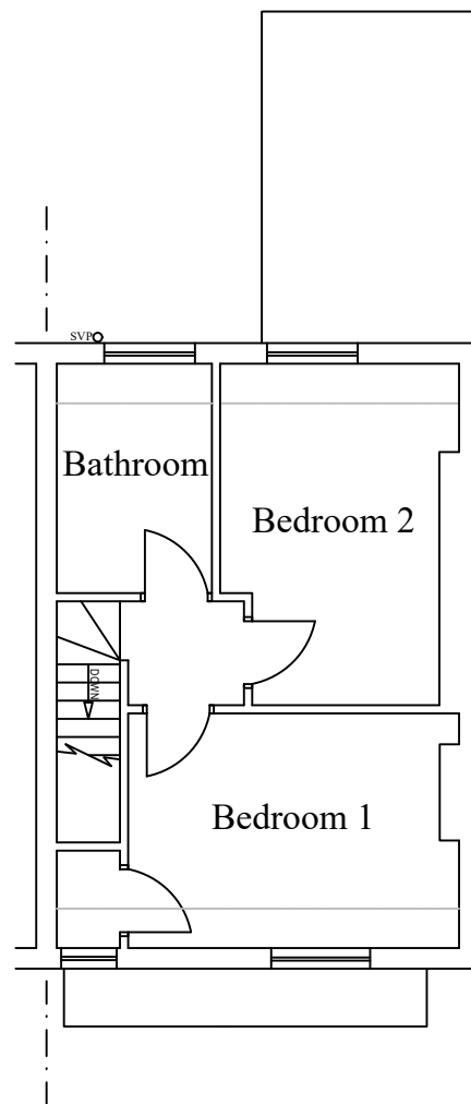
EXISTING FIRST FLOOR LAYOUT
