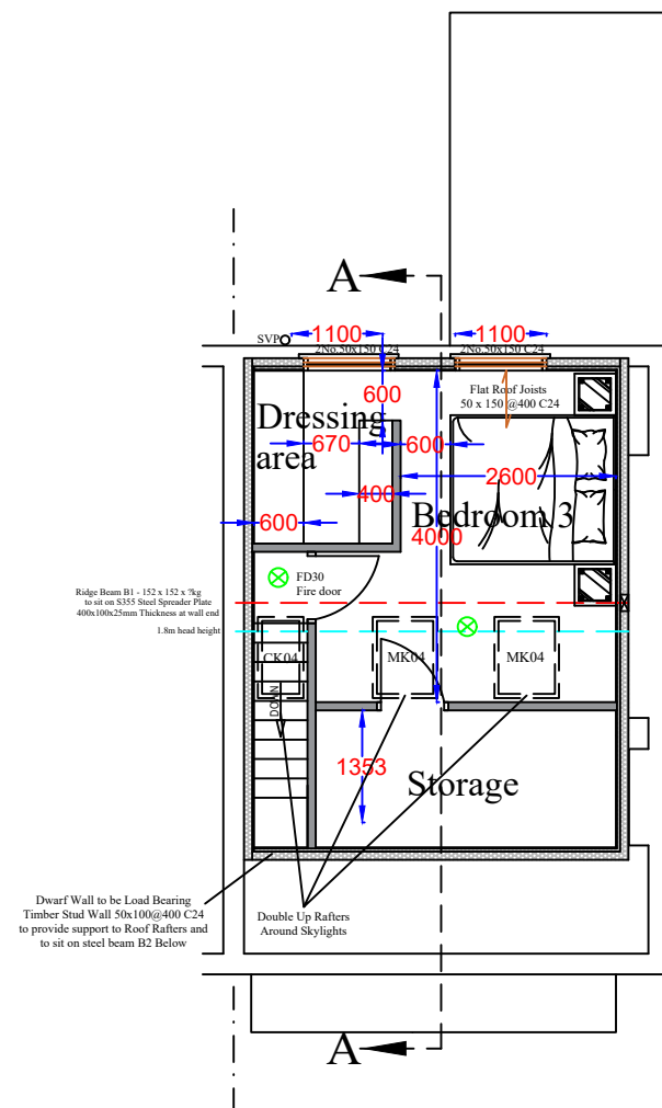
PROPOSED LOFT FLOOR LAYOUT
