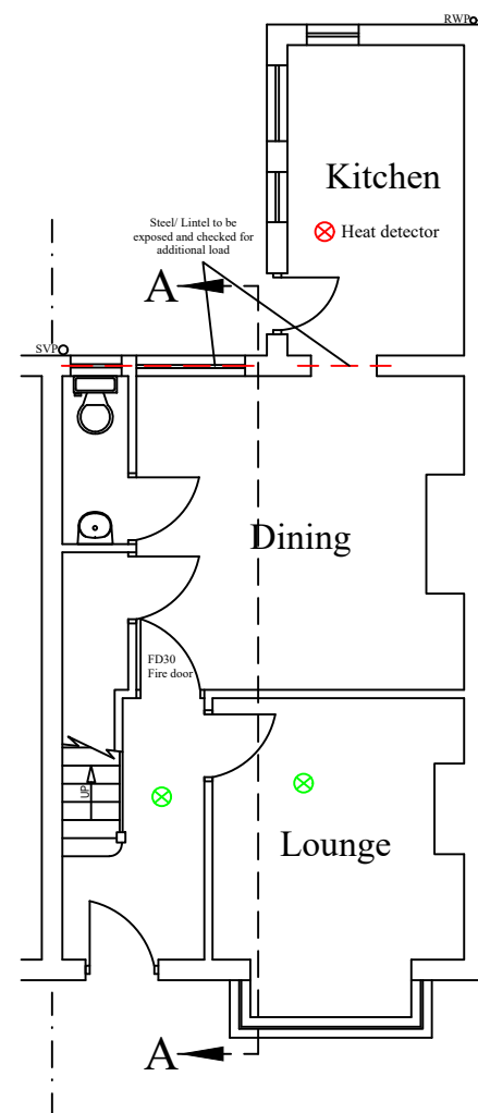
PROPOSED GROUND FLOOR LAYOUT
