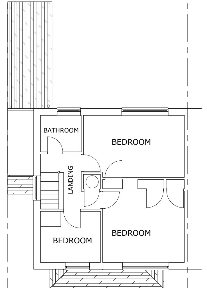
FIRST FLOOR
