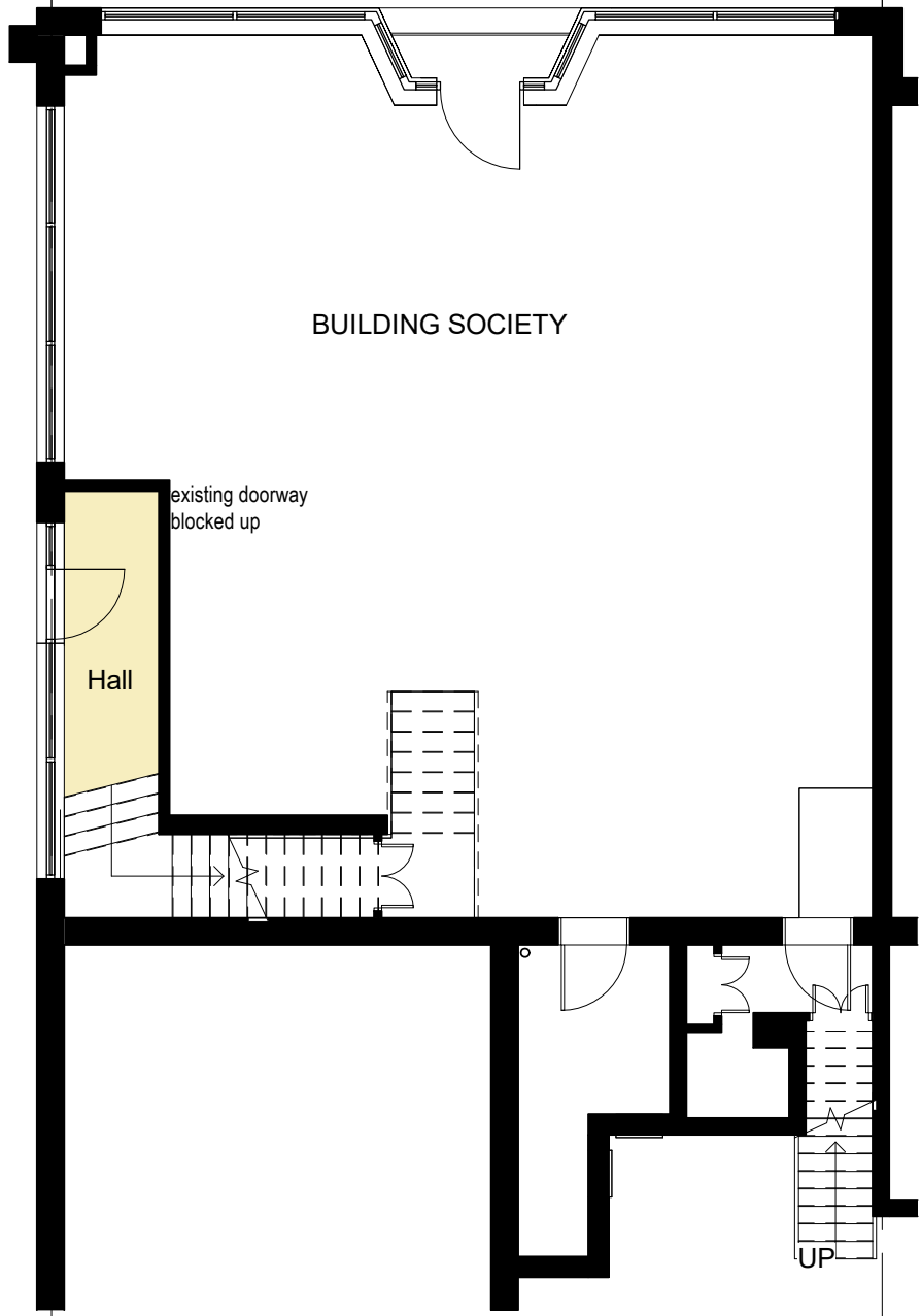
Proposed Ground Floor 1 : 100
