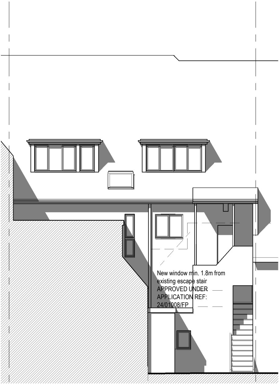
Proposed North Elevation 1 : 100
