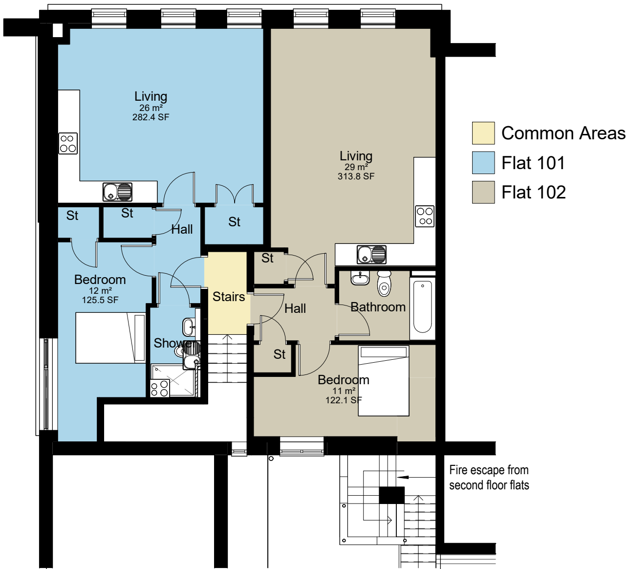
Proposed First Floor 1 : 100 CHANGE OF USE OF FIRST FLOOR APPROVED UNDER APPLICATION REF: 24/01008/FP
