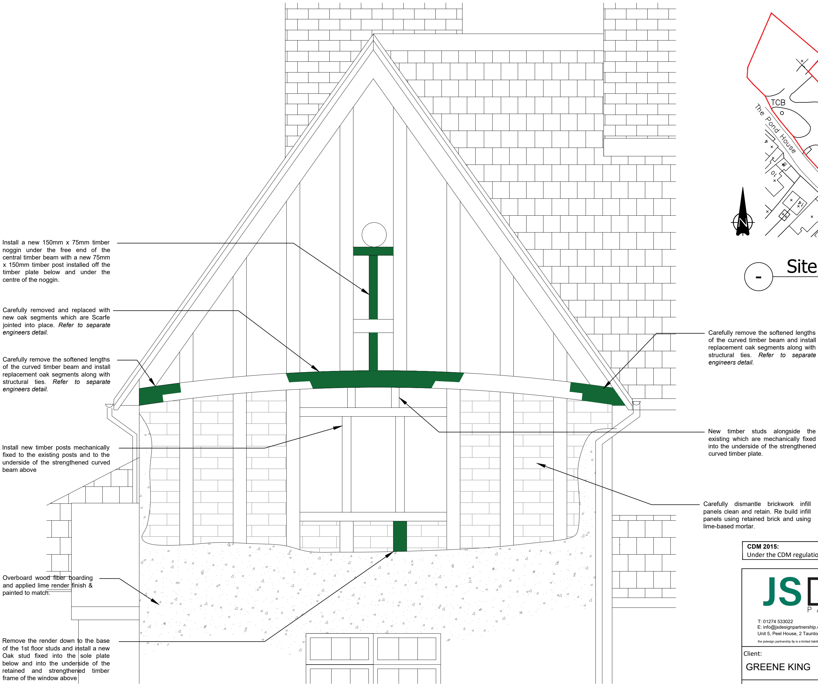
4 Proposed Gable Scale: 1:20
