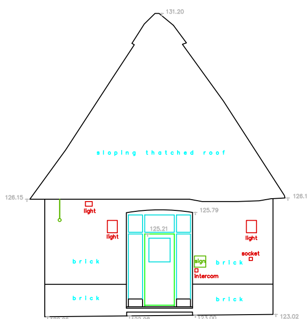
ELEVATION D
