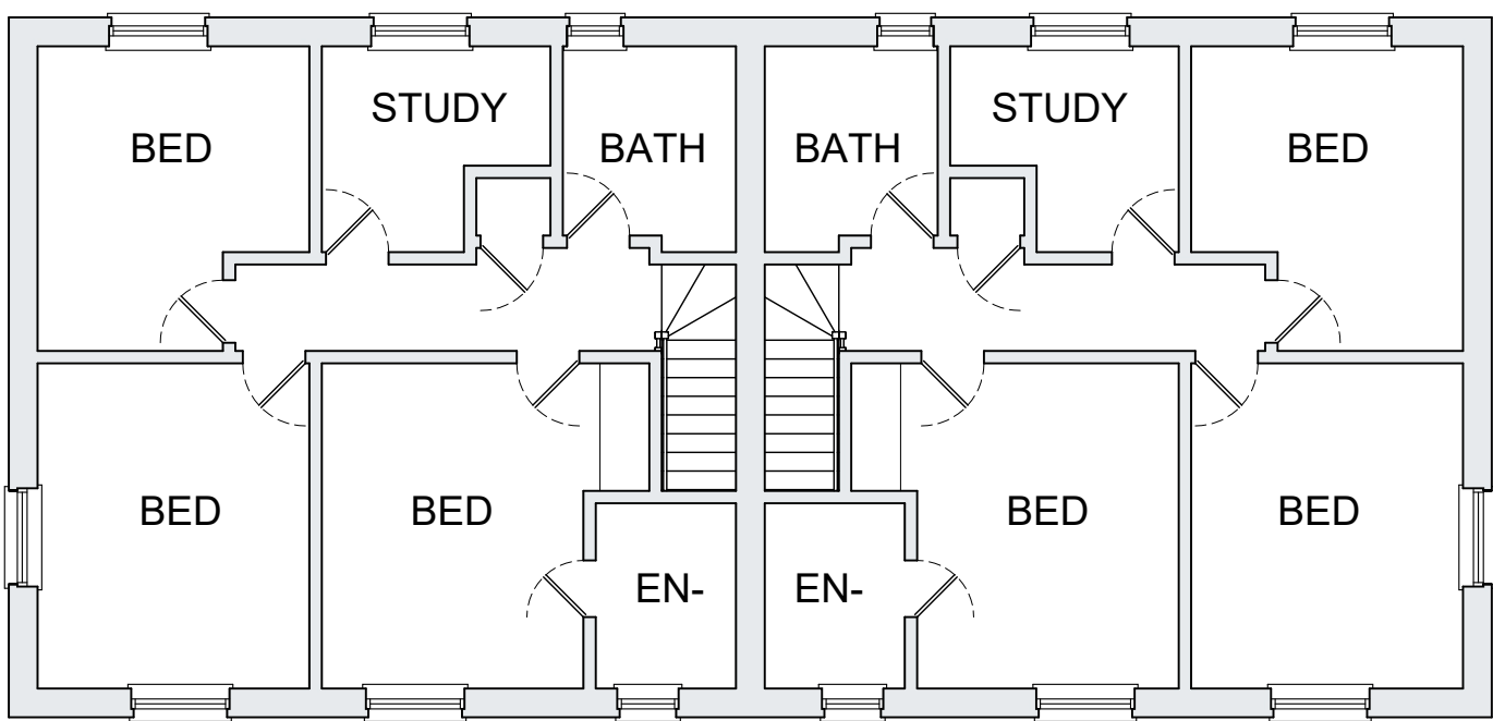
FIRST FLOOR 1:100
