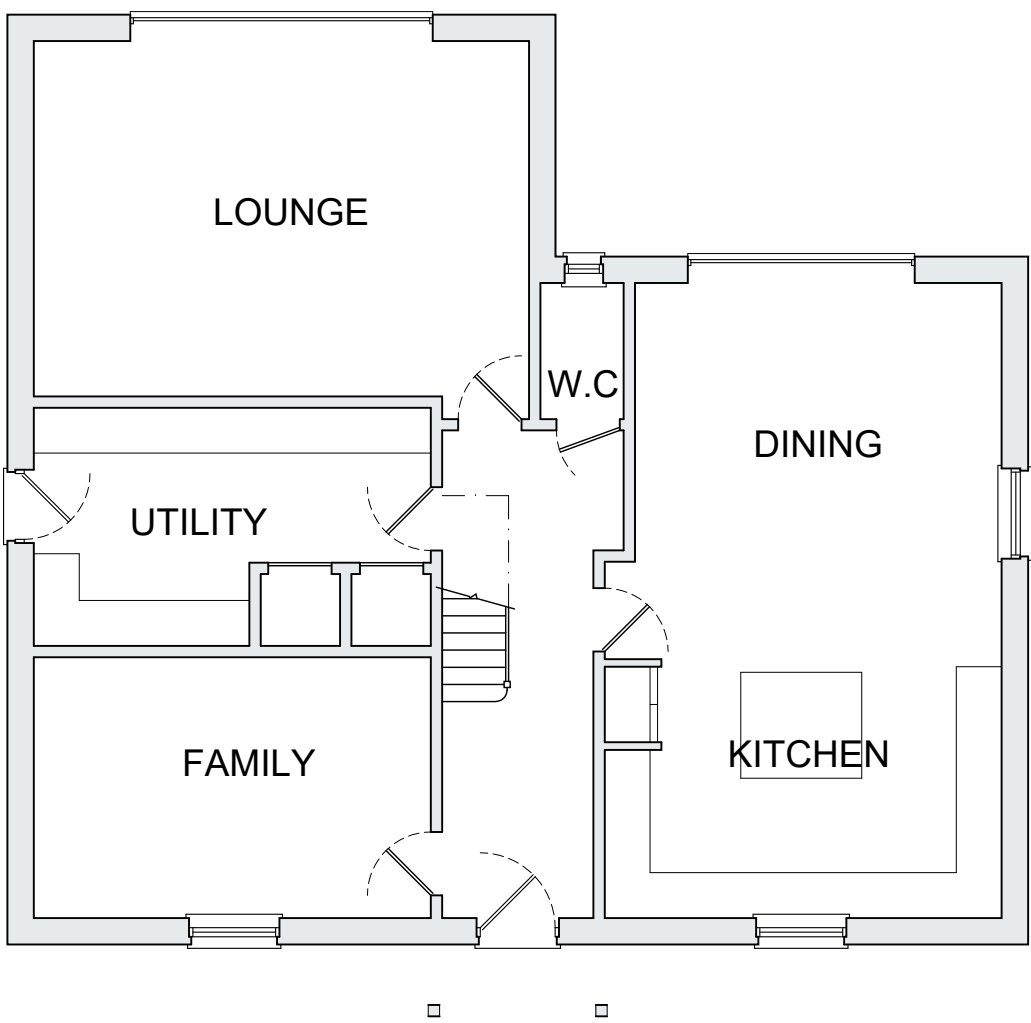
GROUND FLOOR 1:100 PLOT 5
