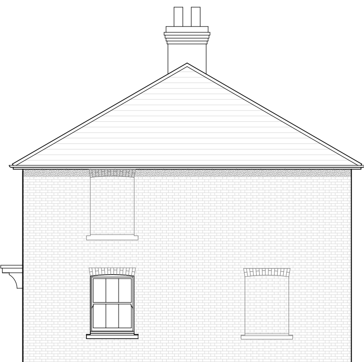
SOUTH ELEVATION 1:100
