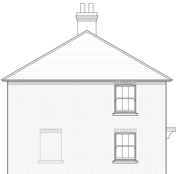
NORTH ELEVATION 1:100 PLOTS 6 & 7
