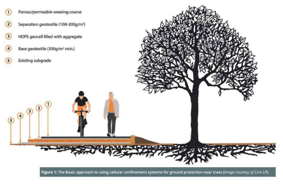
Figure 1: The basic approach to using cellular confinement systems for ground protection near trees [image courtesy of Core LP]
