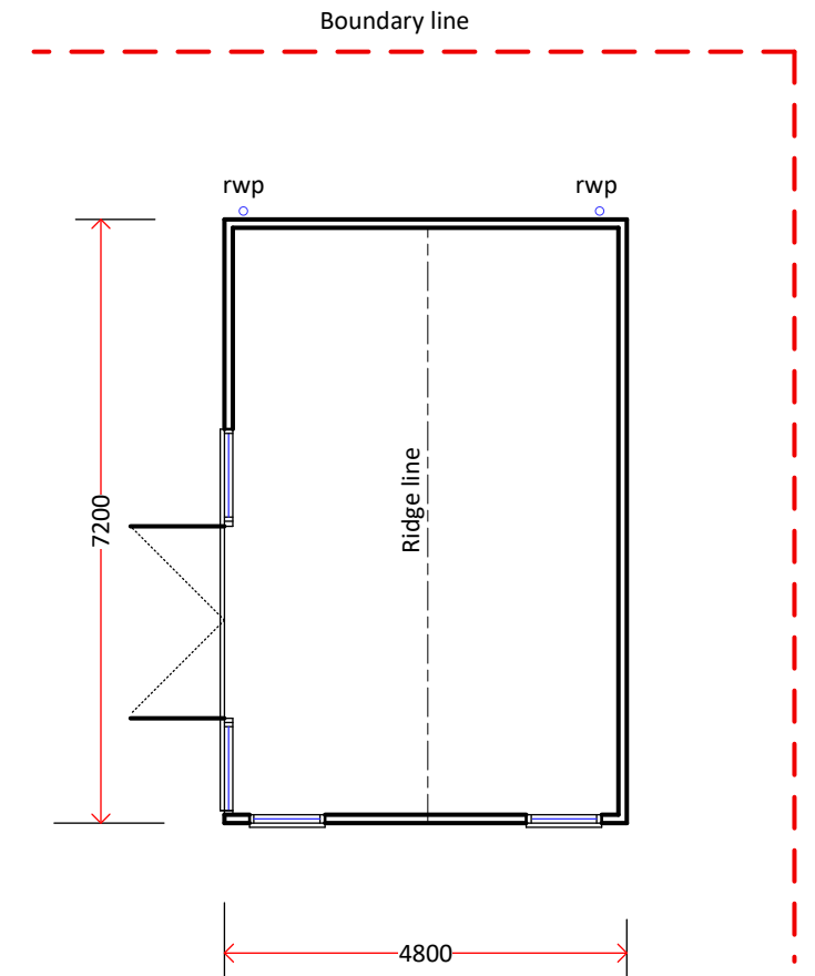
GF PLAN
