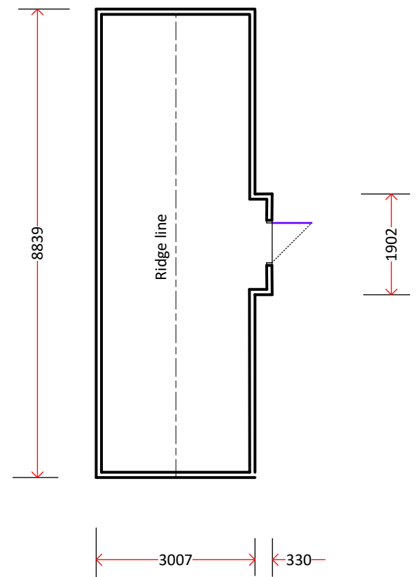
GF PLAN
