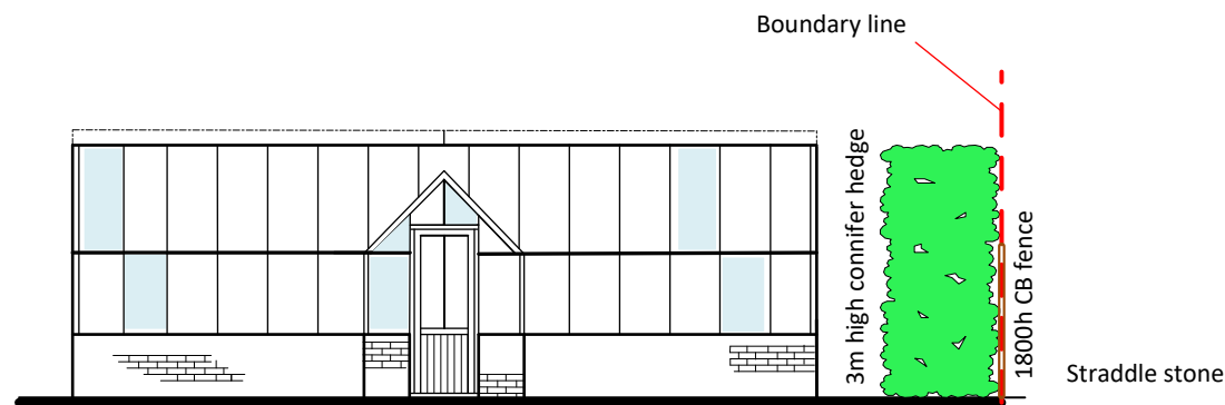
FRONT – view from pool
