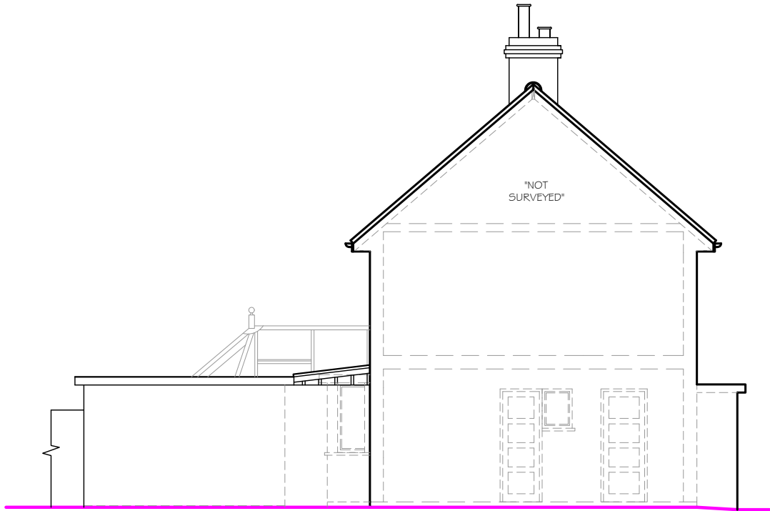
EXISTING SIDE ELEVATION 01
