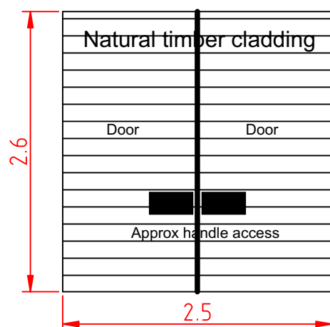
West Elevation
