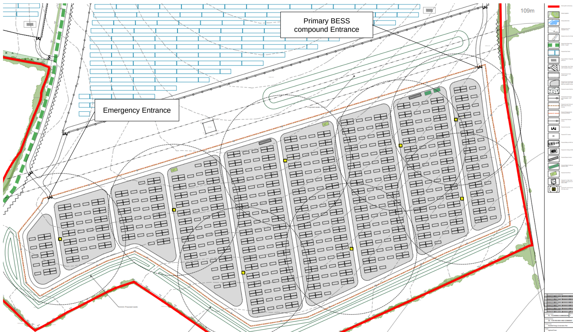
Figure 5-3 Westfield Energy Conservation Park Proposed BESS Compound Layout
