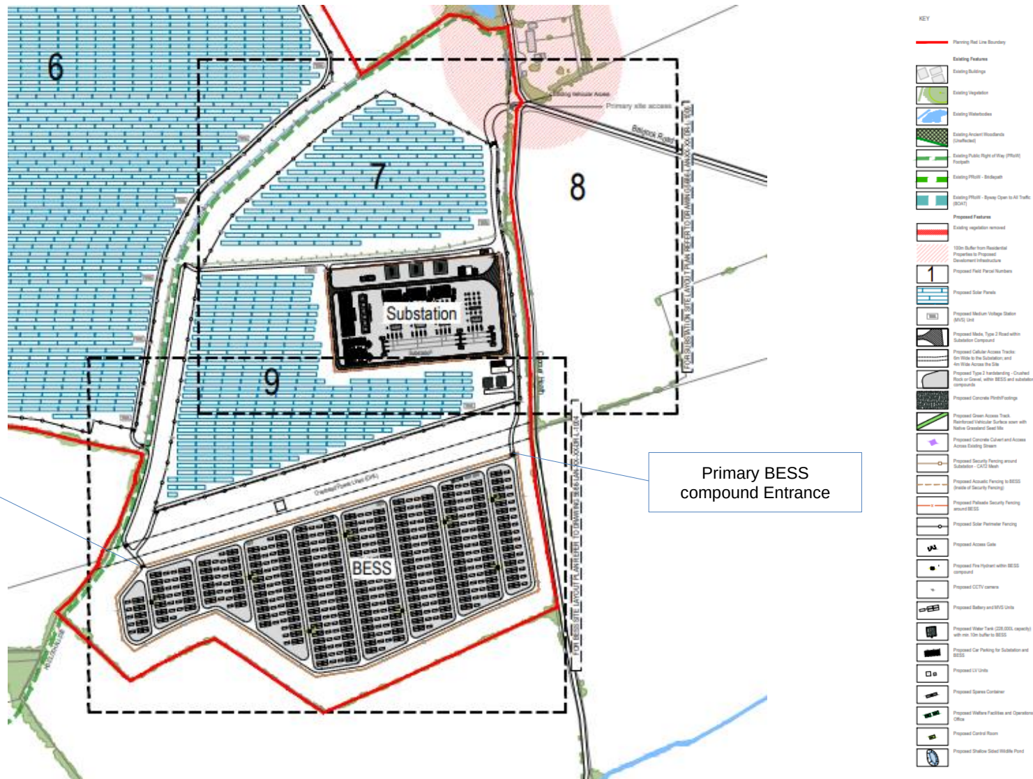
Figure 5-2 Westfield Energy Conservation Park Site Layout (Eastern Element only)
