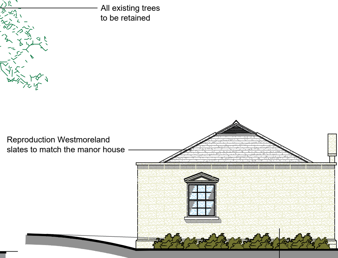
East
