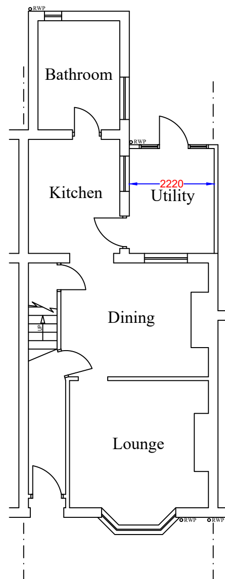
EXISTING GROUND FLOOR LAYOUT
