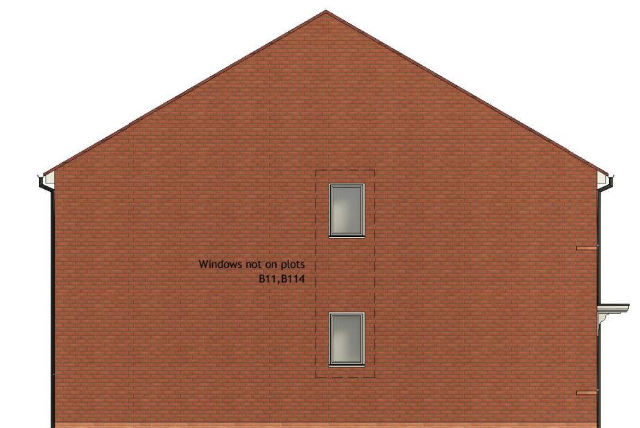
Left Elevation
