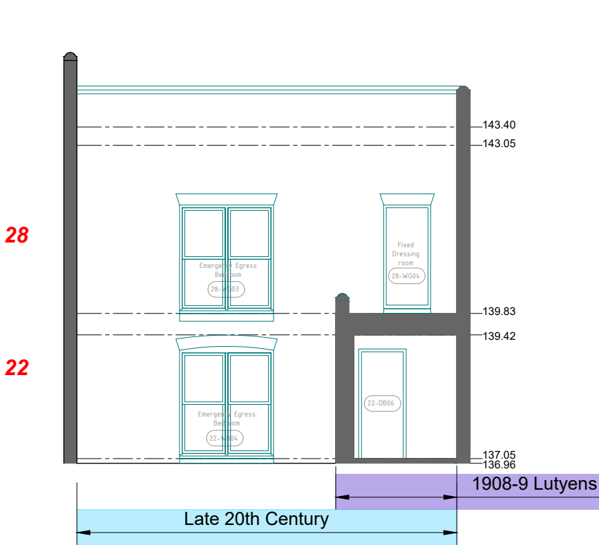
B Proposed Courtyard North Elevations ~ 12004
