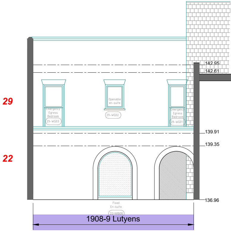
C Proposed Courtyard East Elevations ~ 12004
