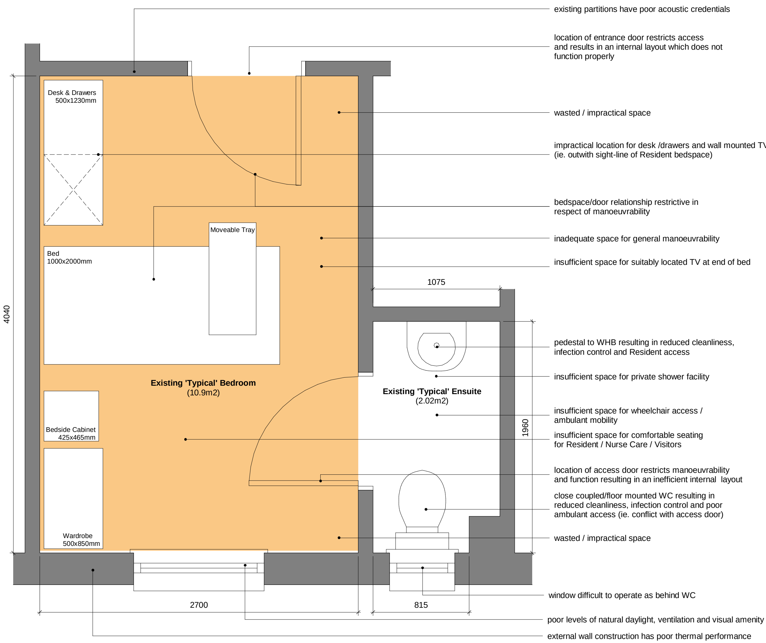
Existing 'Typical' Bedroom (10.9m2 Bedroom with 2.02m2 Ensuite) 1 : 20
