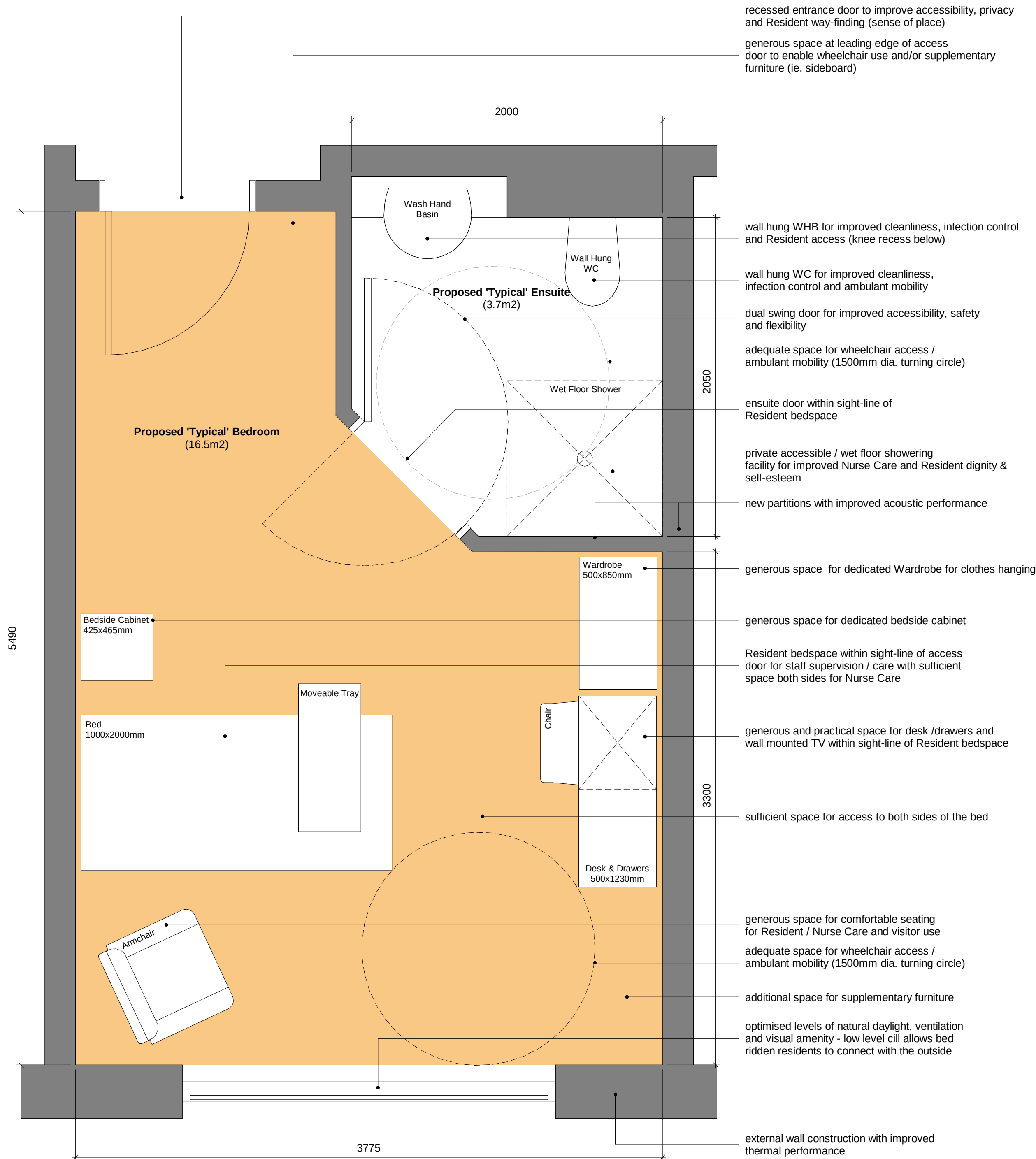
Proposed 'Typical' Bedroom (16.5m2 Bedroom with 3.7m2 Ensuite) 1 : 20
