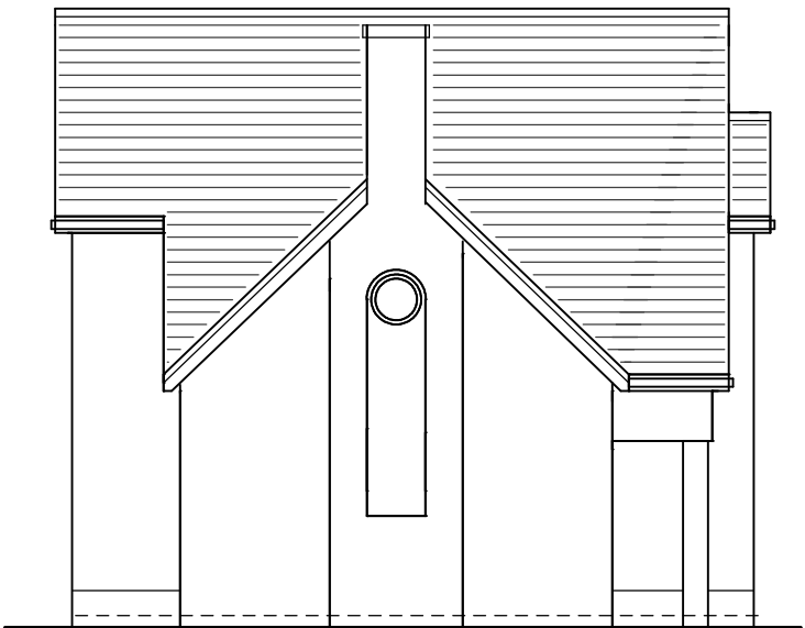
left side (northeast) elevation
