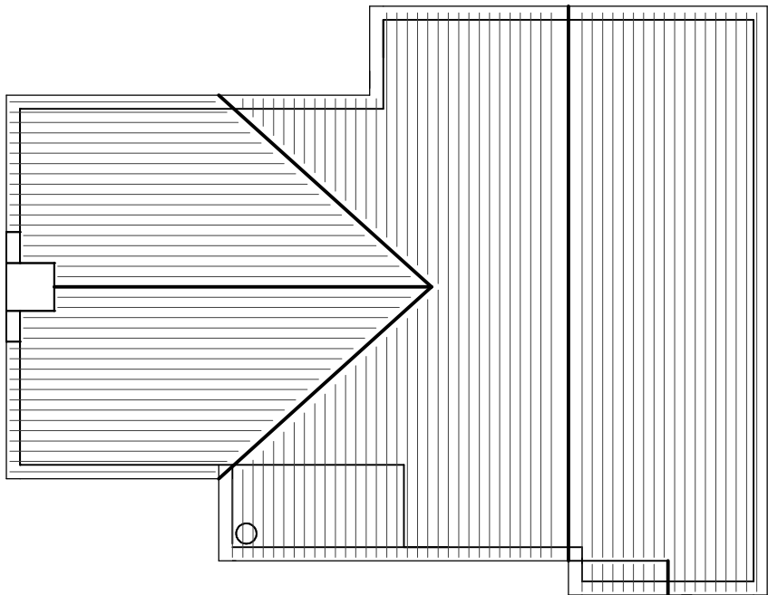
ROOF PLAN
