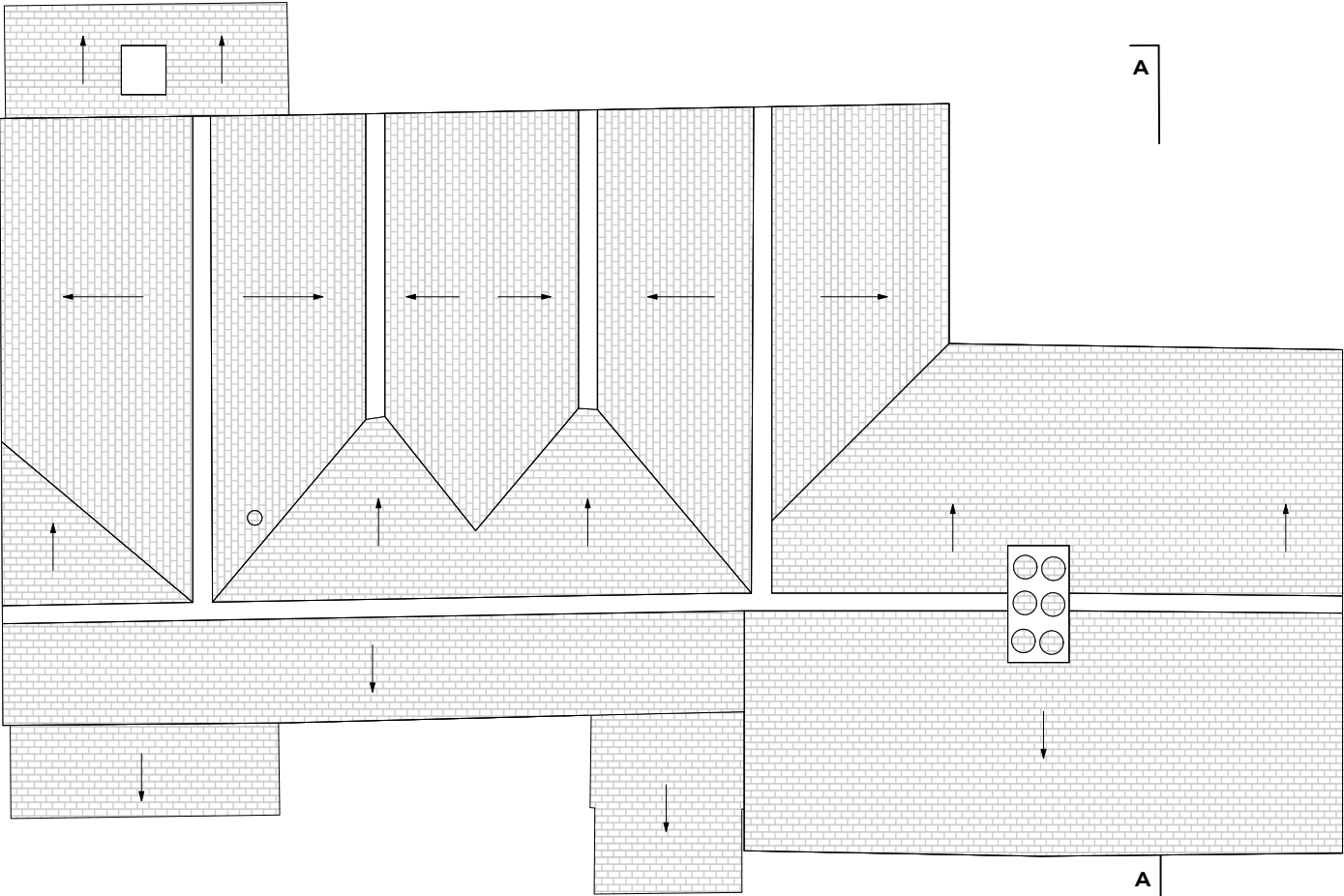
Roof Plan 1:100
