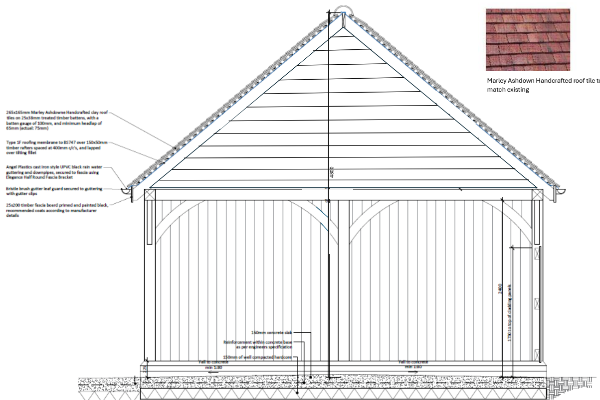
Proposed Section A-A 1:20
