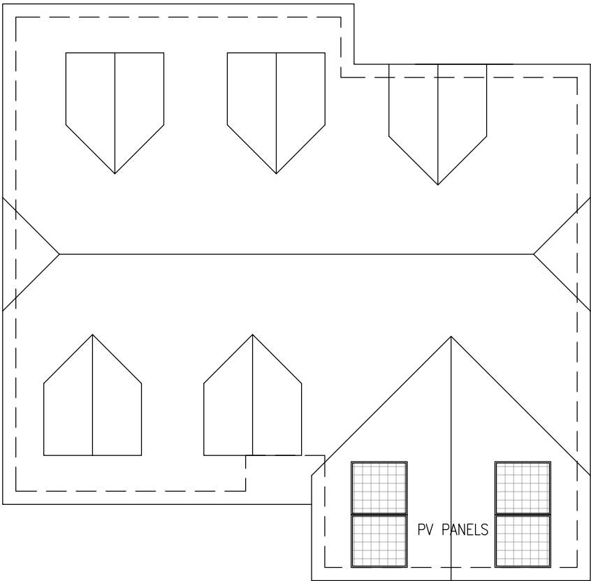
Roof Plan @ 1/100
