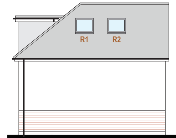
Side Elevation (South)
