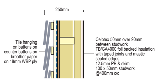
Dormer Wall Detail U=0.18
