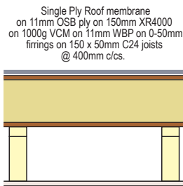
Flat Roof U=0.15
