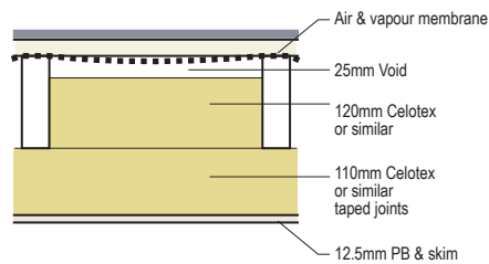
Sloping Ceiling Detail U=0.11
