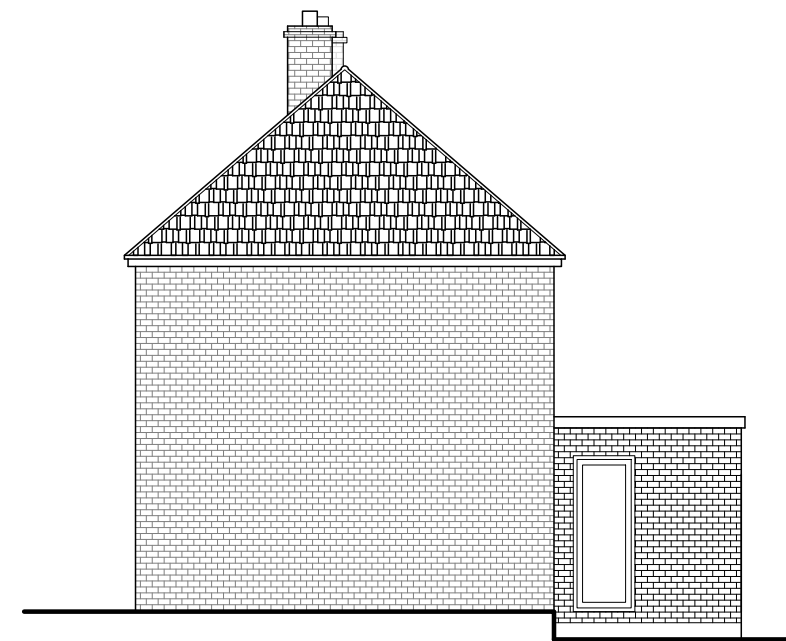
02 A-307 PROPOSED RIGHT ELEVATION SCALE- 1:100@A3
