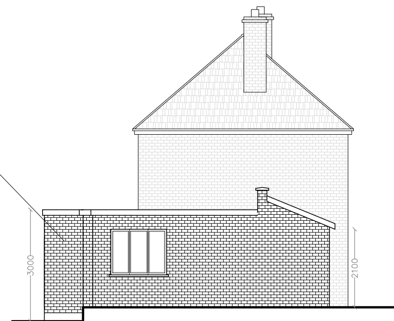
03 A-307 PROPOSED LEFT ELEVATION SCALE- 1:100@A3
