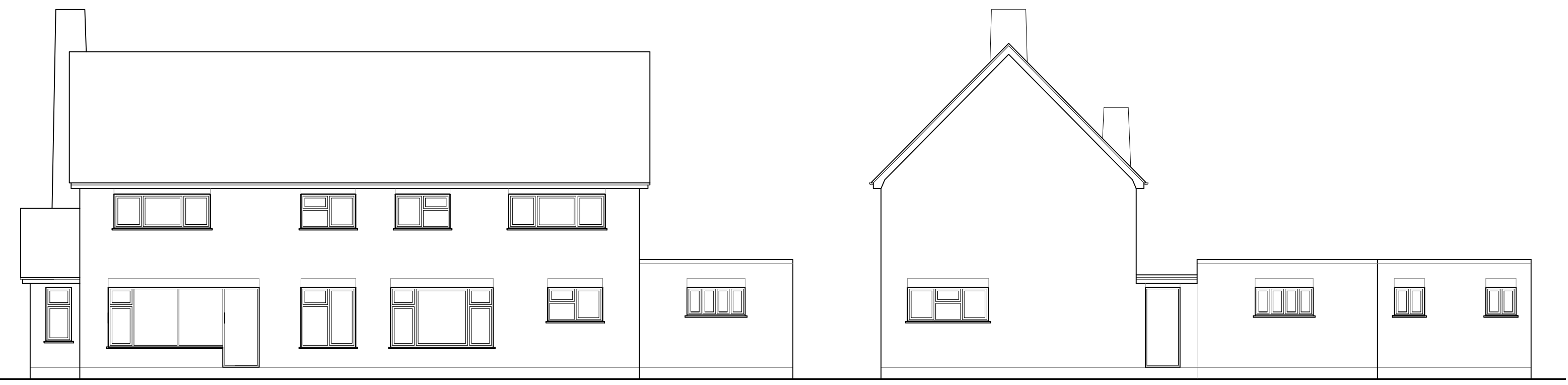
REAR ELEVATION
