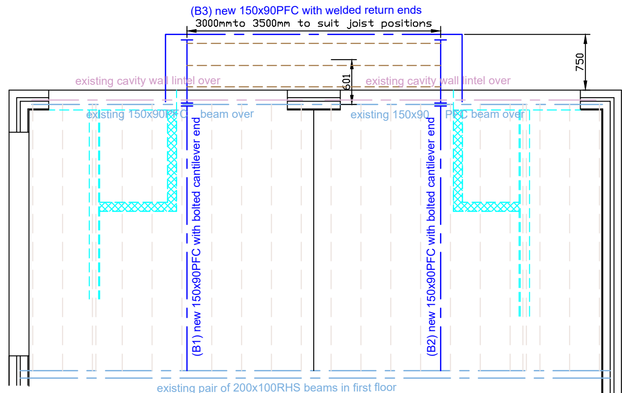
Existing Ground Floor showing new beams over
