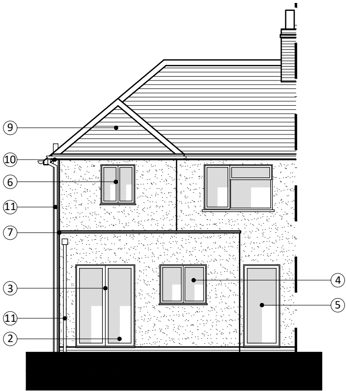
REAR ELEVATION (C-C)
