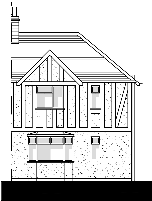
FRONT ELEVATION (A-A)
