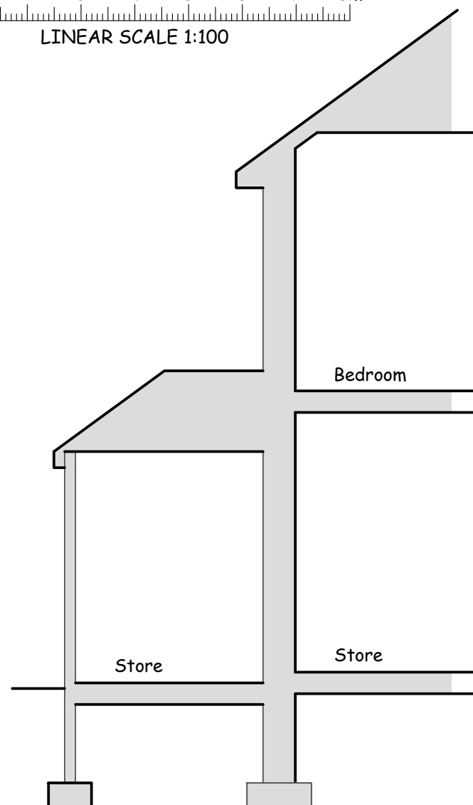
Existing Section 1:50
