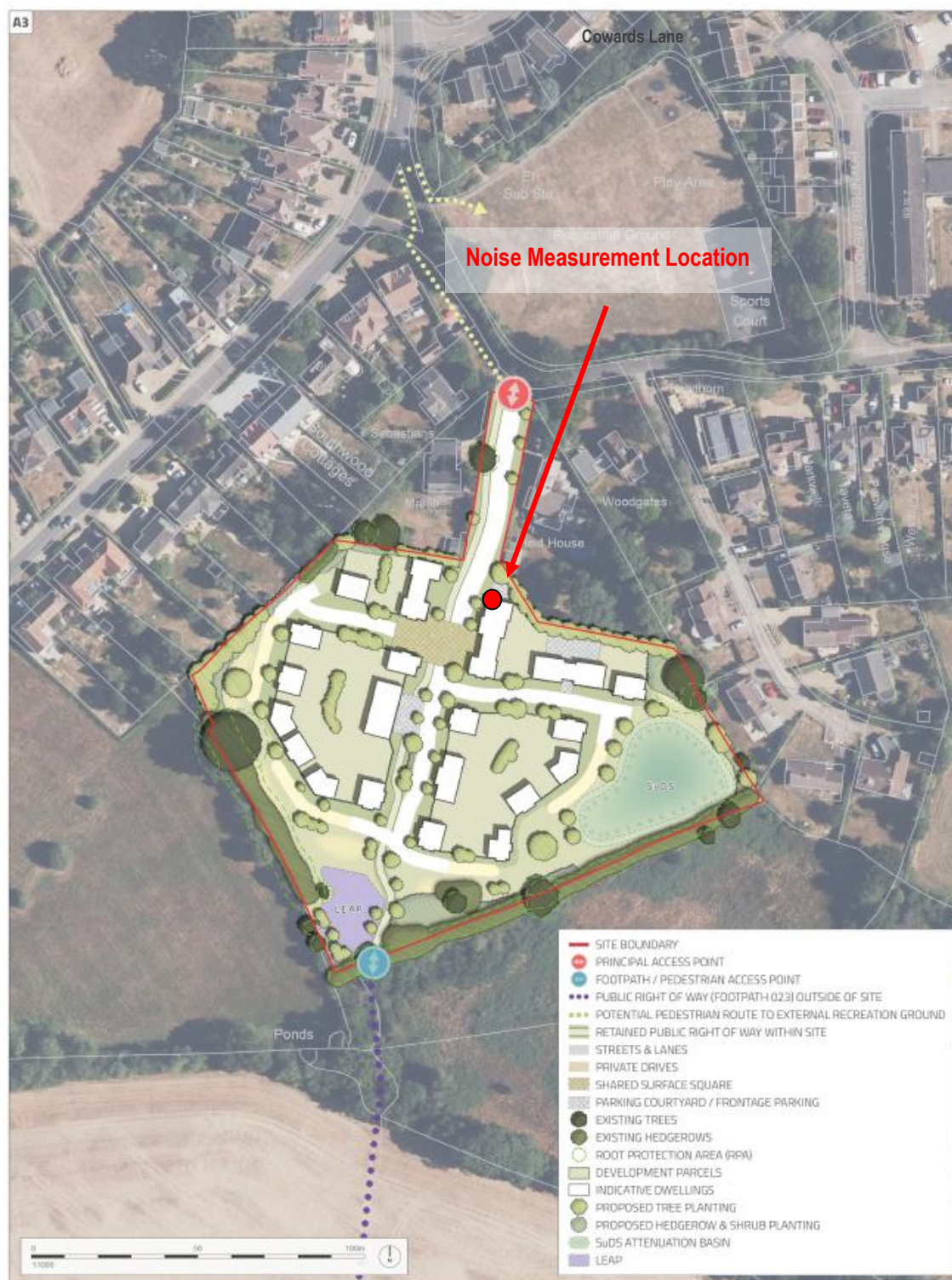
Figure 4.1: Noise Measurement Location &amp; Proposed Site Plan
