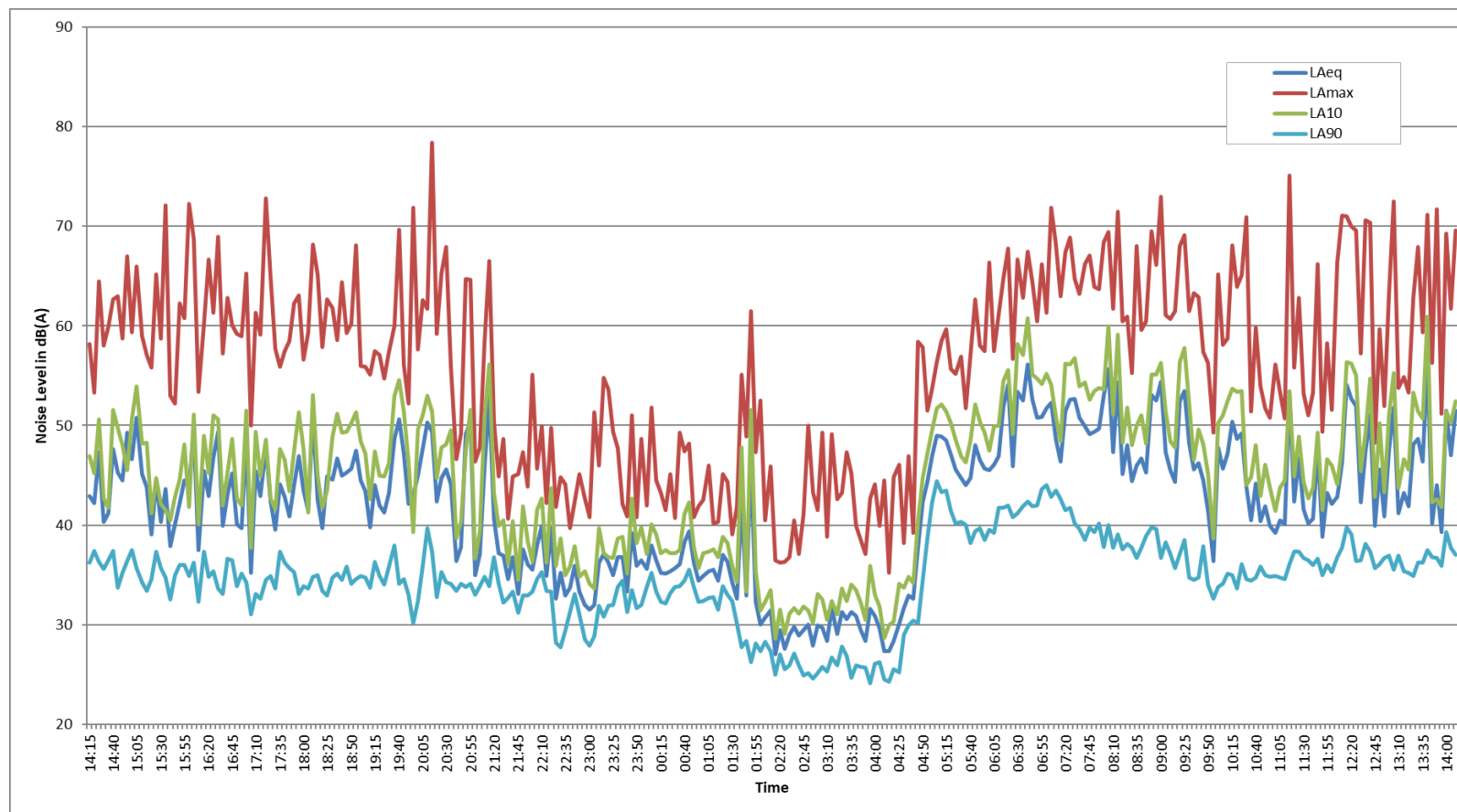
Figure 4.2: Noise Measurements
