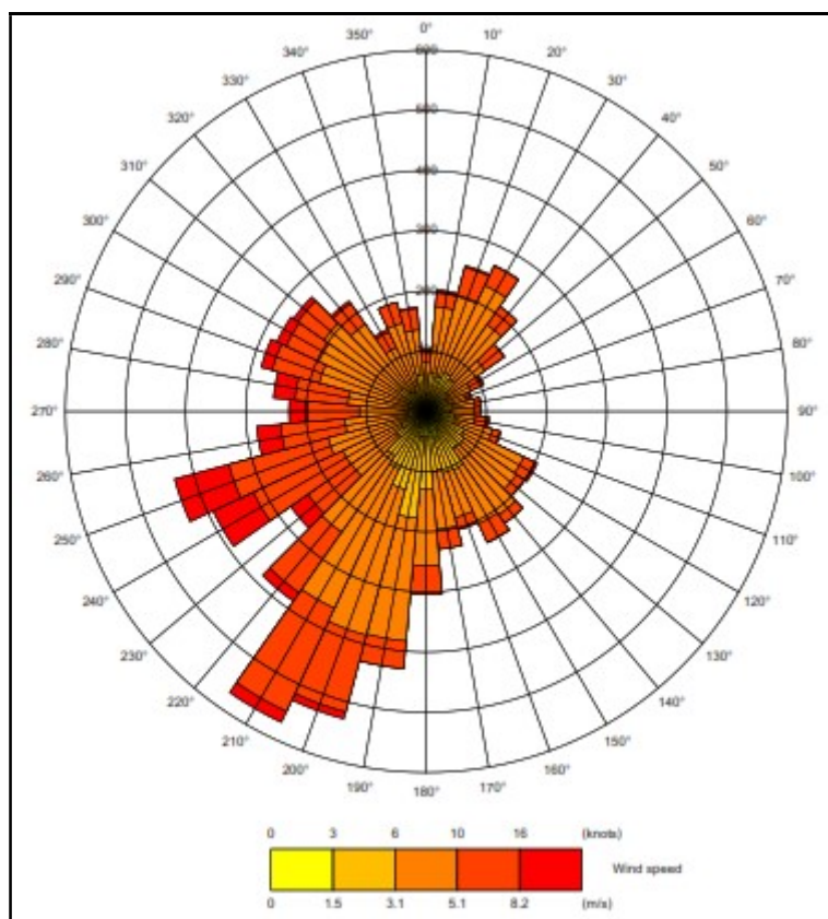
Figure 5.1: Wind Rose for Luton Meteorological Station
