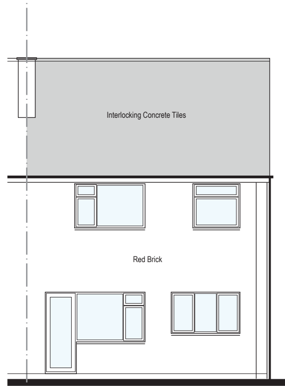
Rear Elevation
