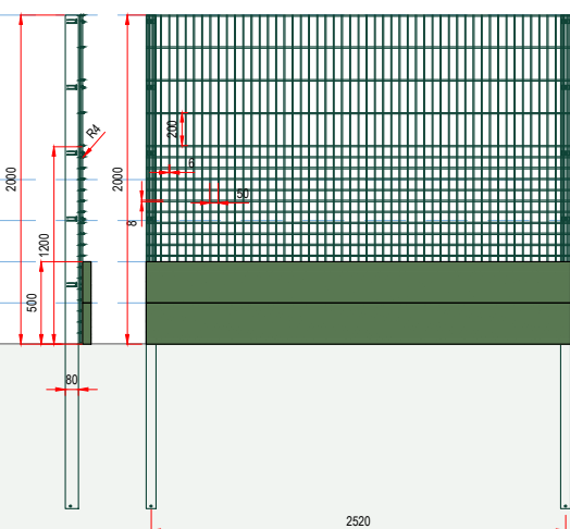
2.0m site perimeter fence
