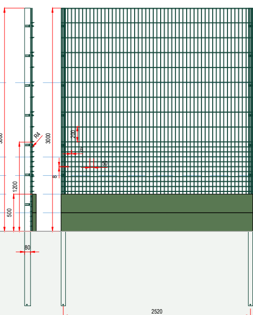
3.0m site perimeter fence
