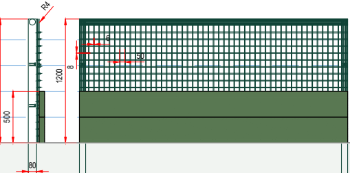
1.2m pitch perimeter fence
