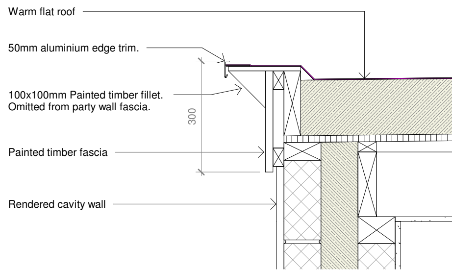
2 Typical Fascia Detail. 1 : 10
