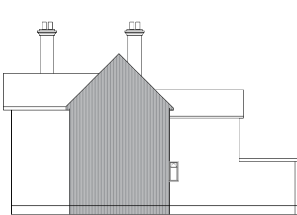
SIDE ELEVATION THROUGH PARTY WALL
