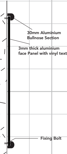
C ONE X NEW AMENITY BOARD WITH SCUMBLE BACKBOARD AND VINYL DETAILING. SIZE. 1.2m x 800mm. H.A.G. 1.2m.
