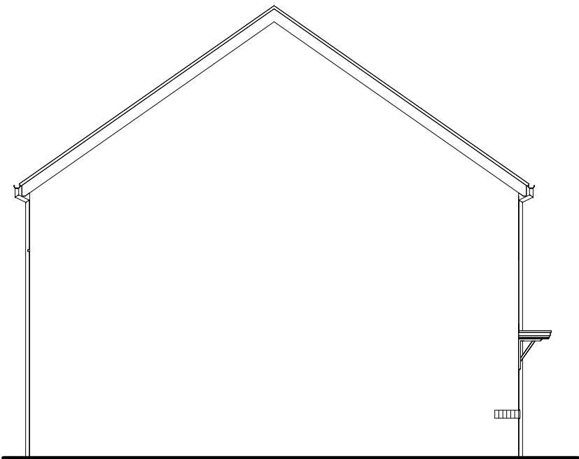
Left Elevation
