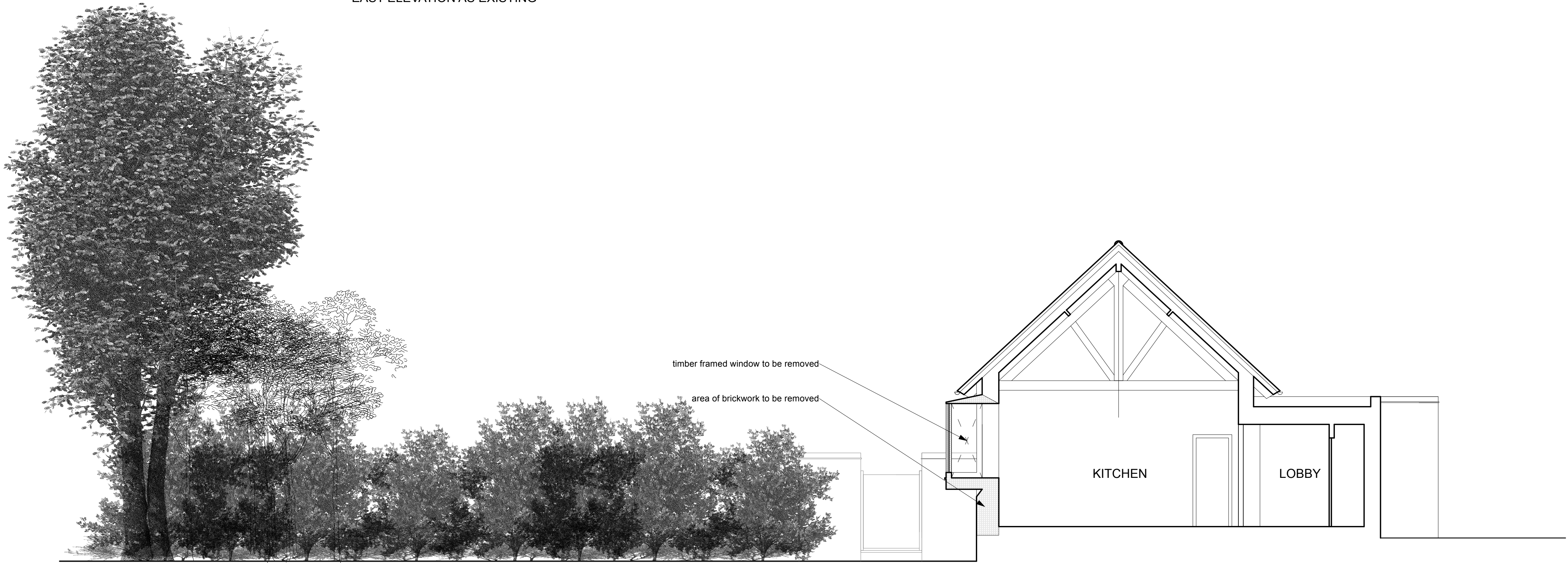
EAST ELEVATION AS EXISTING
