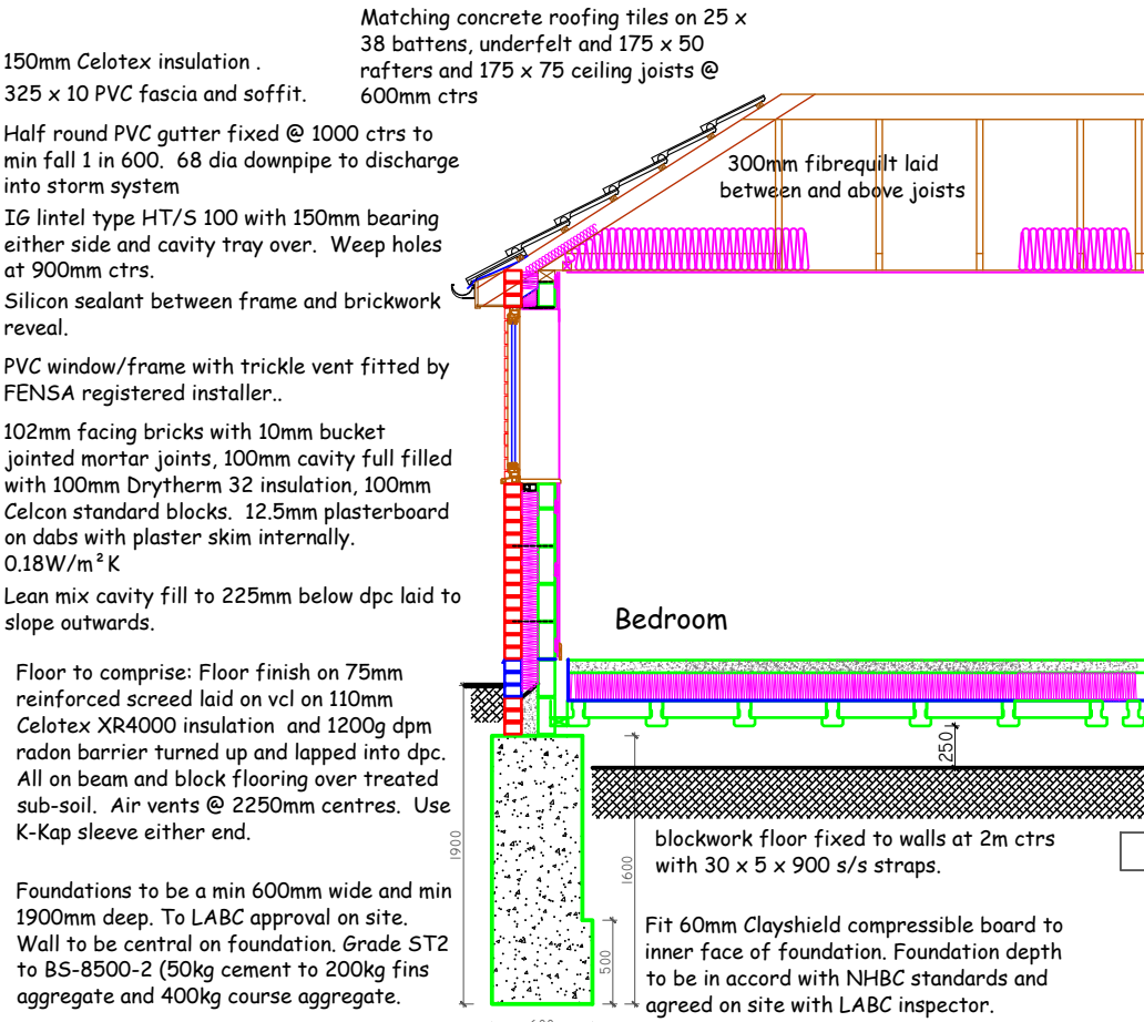
Proposed Section 1:50
