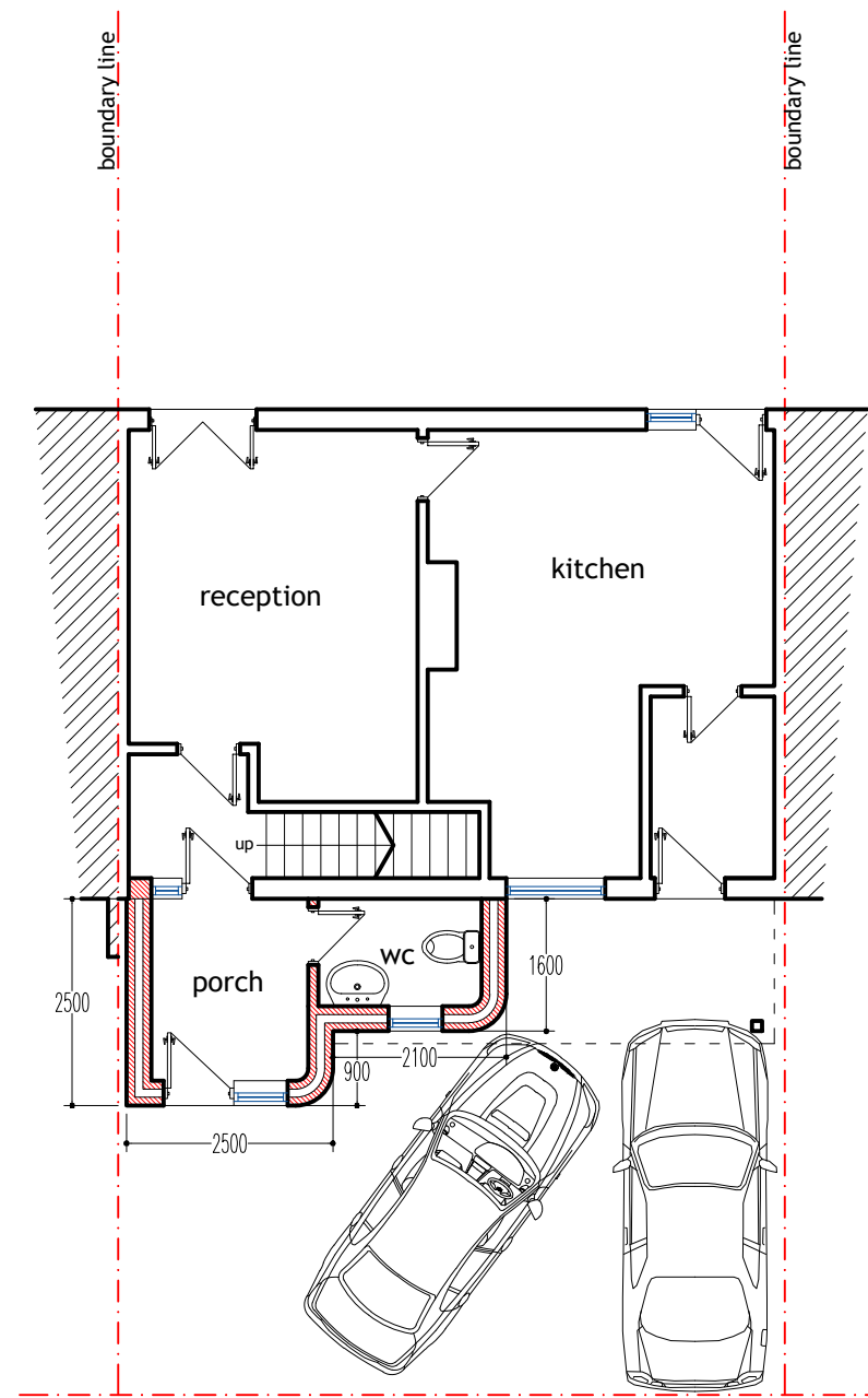
proposed plan
