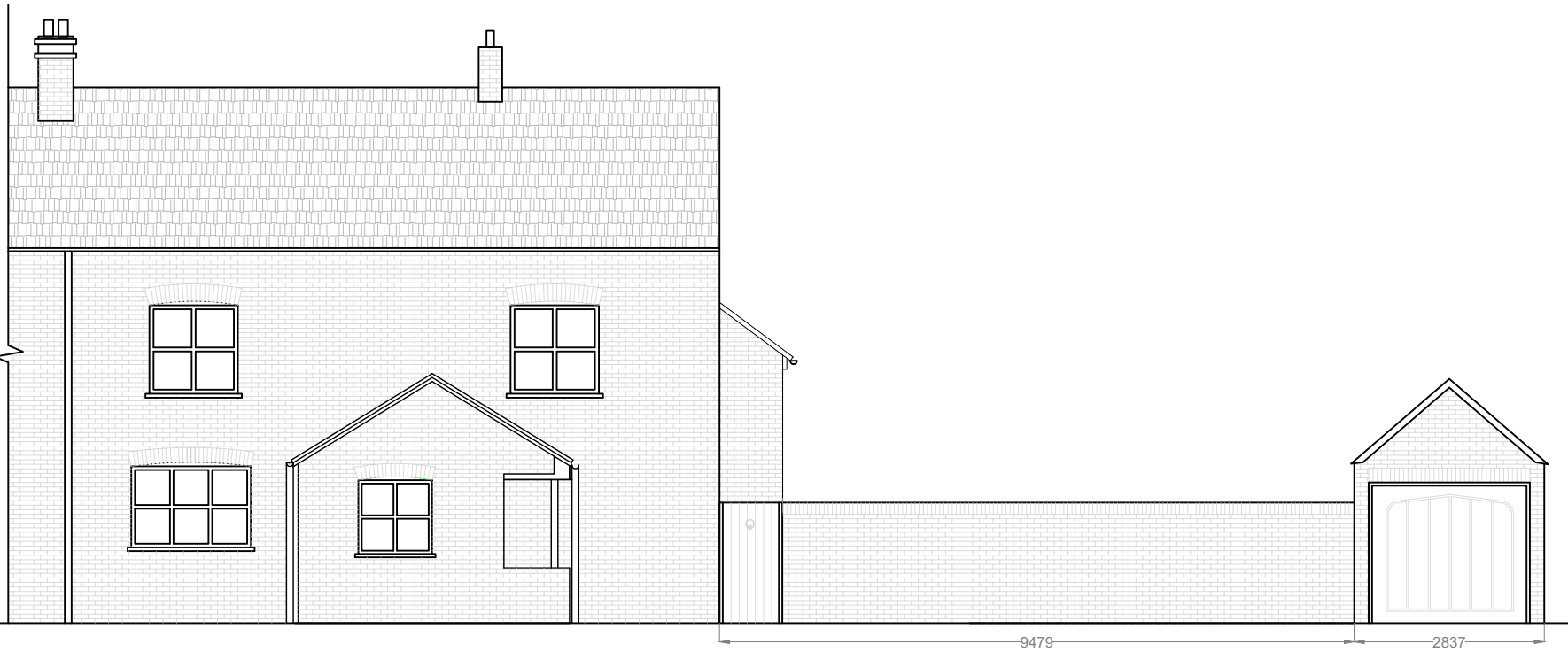
West Elevation— Existing
