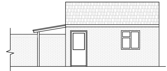
North Elevation — Existing
