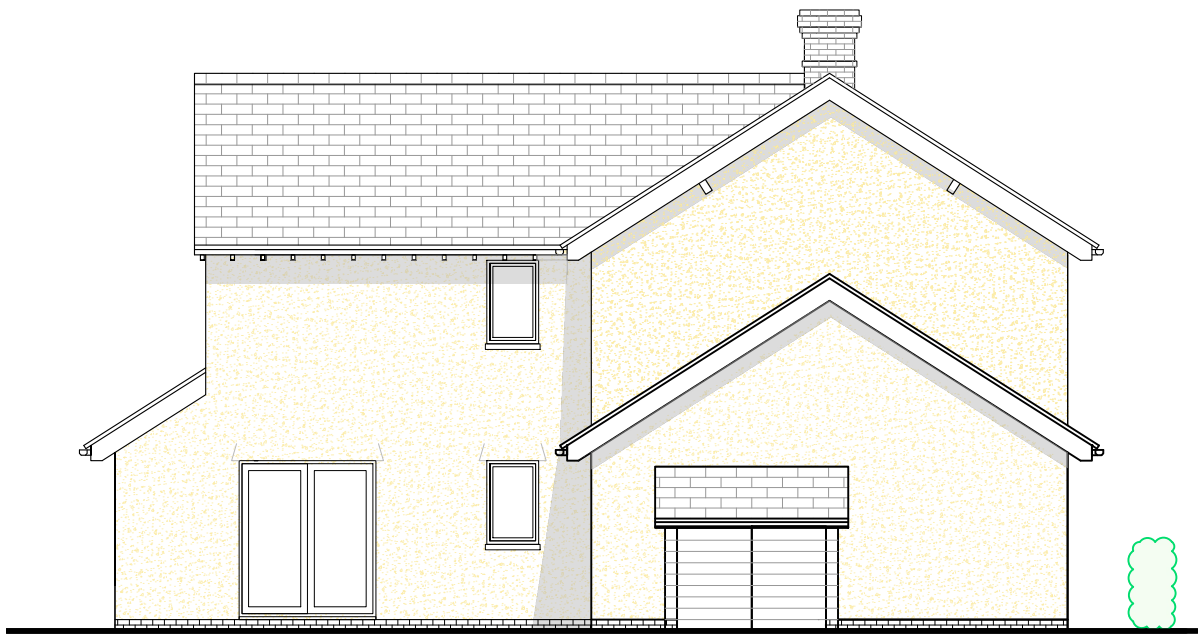
South Elevation - Facing Lodge Cottage
