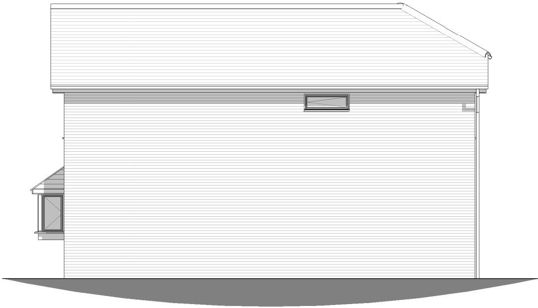
Existing Elevation Side B 1 : 100
